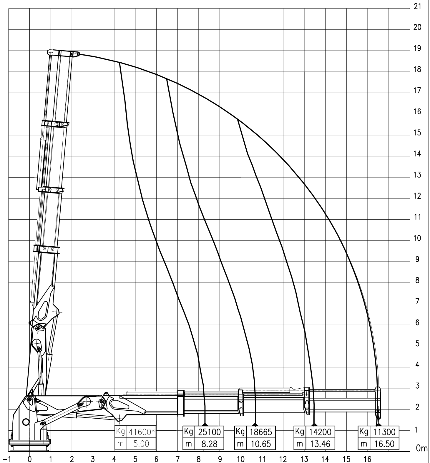
Marine Crane model AKC 290 LHE3 Crane built and designed in according to DIN 15018 Class H1-B3
