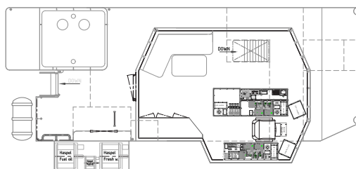
TOPVIEW ON SUPERSTRUCTUREDECK
