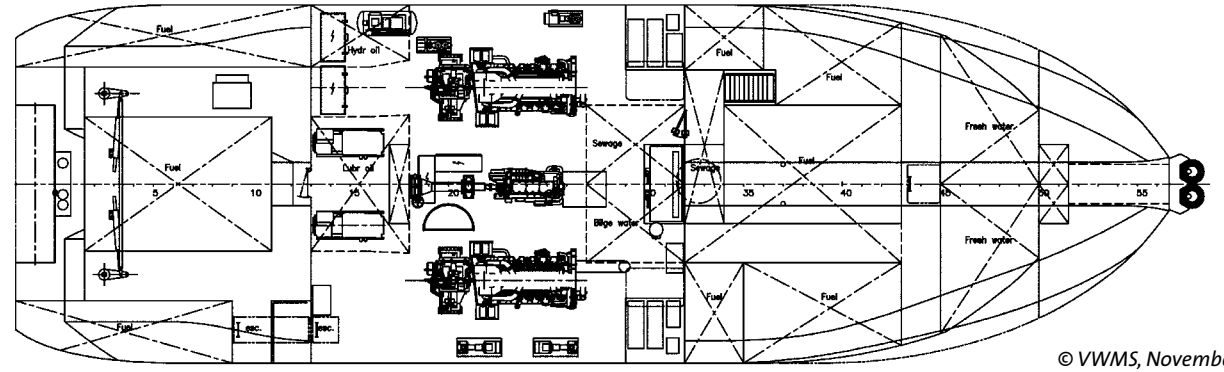
Below maindeck
