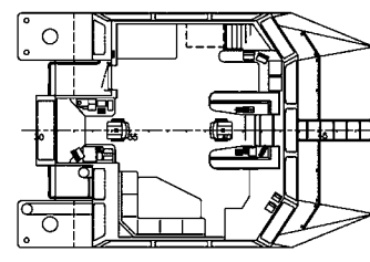
Wheelhousedeck
