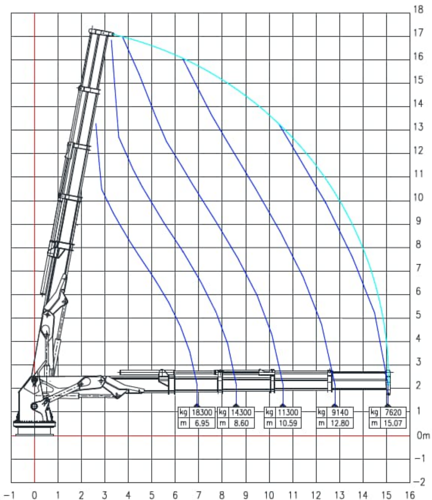
Marine Crane model AKC 185 HE4
